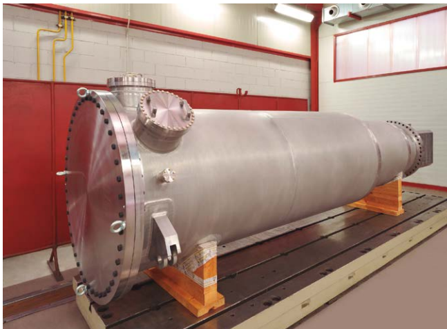
Proton Beam Window Port Block and Proton Beam Window Vessel for European Spallation Source ERIC
