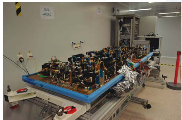
Communications subsystem
