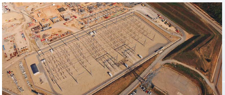
The very high voltage electrical substation on the south side of the platform (Photo IO E3F Richie)
