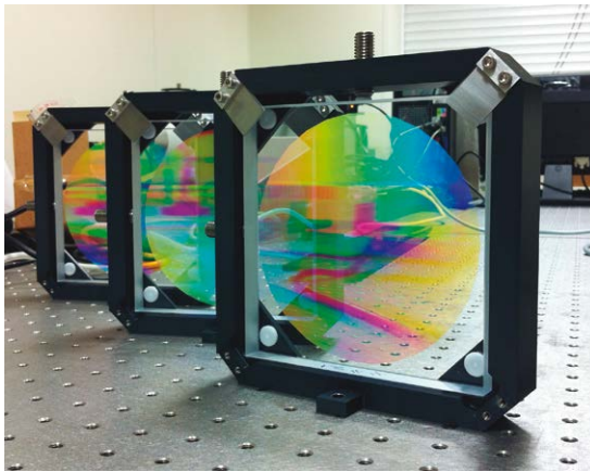
Volume Phase Holographic gratings for ARES spectrograph at Joan Oró telescope(customer IEEC, Barcelona)
