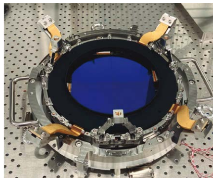
PLATO Focal Plane Assembly CAB_ INTA_LIDAX EM1
