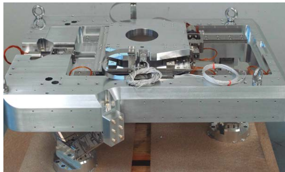
Sub-Micron Positioning System for ESRF ID21 Beamline
