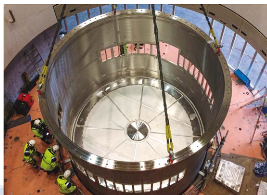
Monolith Vessel Installed in ESS ERIC
