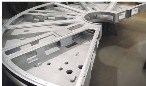
ILL flight vacuum chamber for wasp
