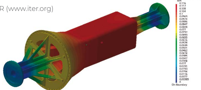
Clessidra dispenser curing tool FEM simulation. Design & Manufacturing.
