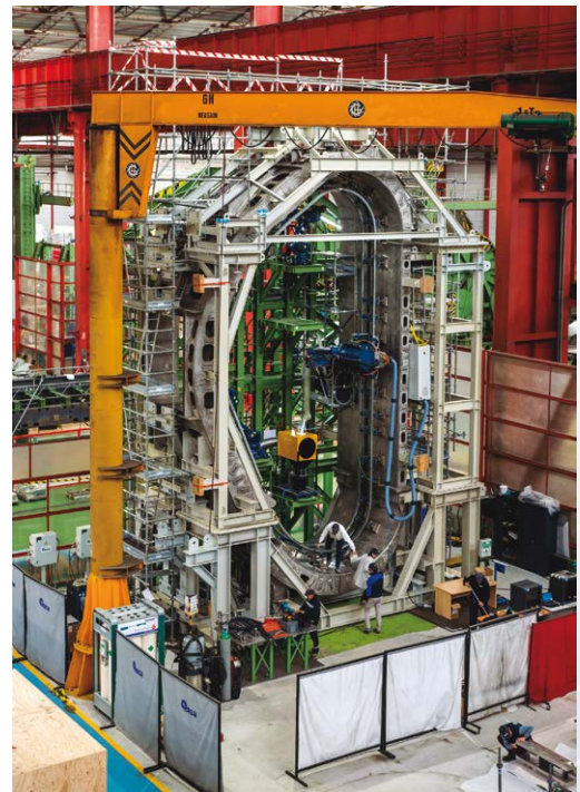
ITER vacuum vessel welding mockup
