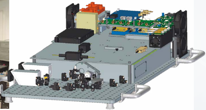
Integrated OEM system for WLCSP (Wafer level chip size packaging)
