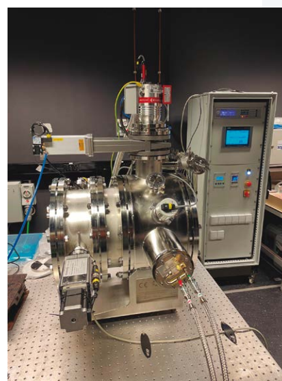
ESA-ESTEC SWIR Bench Cryostat System
