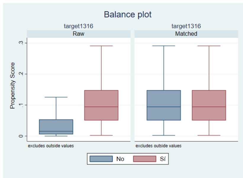
Figure 3: Balance plot before and after matching propensity score (Final eval. matched sample)
