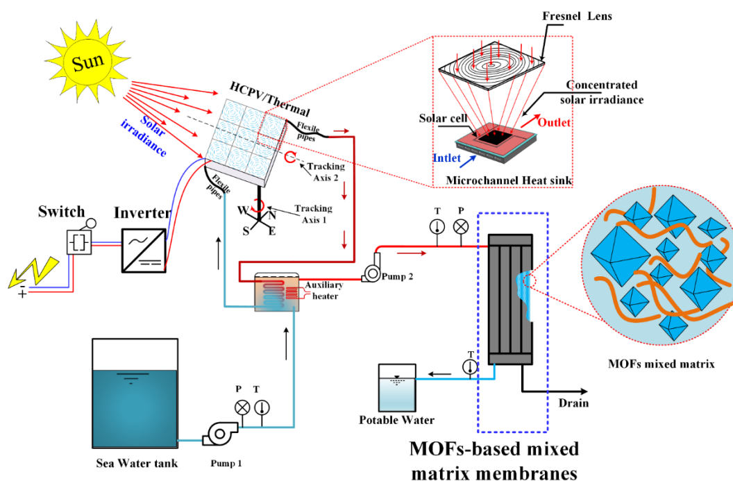
The proposed prototype for a HCPV combined with a MOF membrane desalination system
